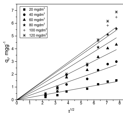
Figure 7. Adsorption kinetic of disperse yellow dye according to the Weber&Morris mechanistic model
